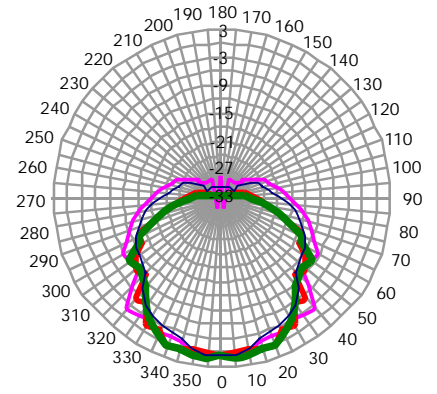
Horizontal polar diagrams
