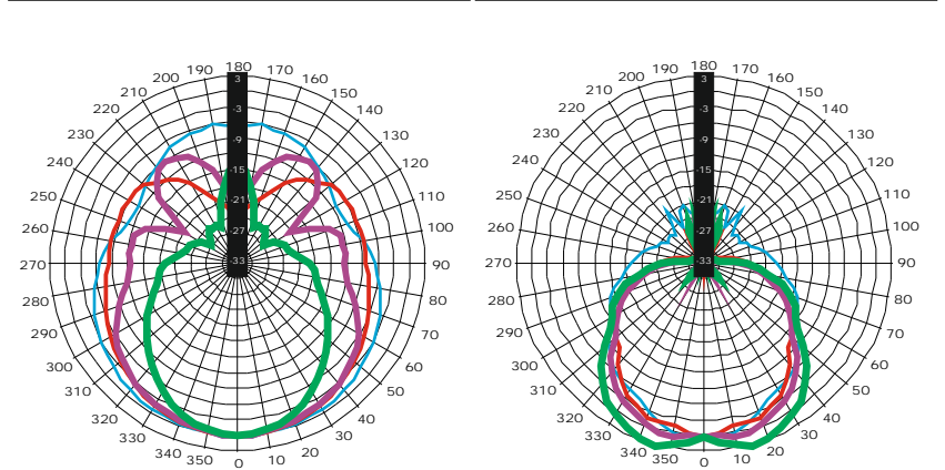
HORIZONTAL POLAR DIAGRAM Legend: 250 (blue), 500 (red), 1000 (purple), 2000 (green), 4000 (cyan), 8000 (orange), 12500 (magenta), 16000 (dark green)
