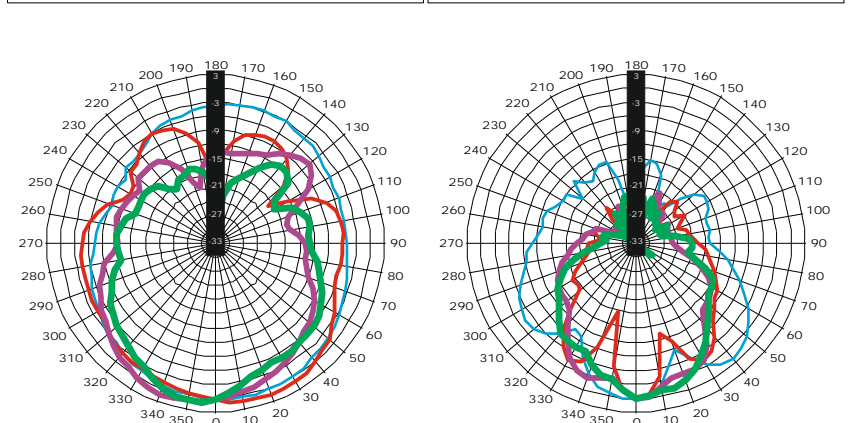
VERTICAL POLAR DIAGRAM Legend: 250 (blue), 500 (red), 1000 (purple), 2000 (green), 1400 (cyan), 2000 (orange), 2500 (magenta), 3150 (dark green)
